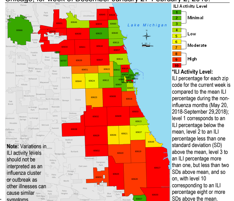
Figure 6. Influenza-like Illness (ILI) activity level by patient zip code determined by chief complaint data submitted to ESSENCE , Chicago, for week of December January 27-February 2, 2019.
